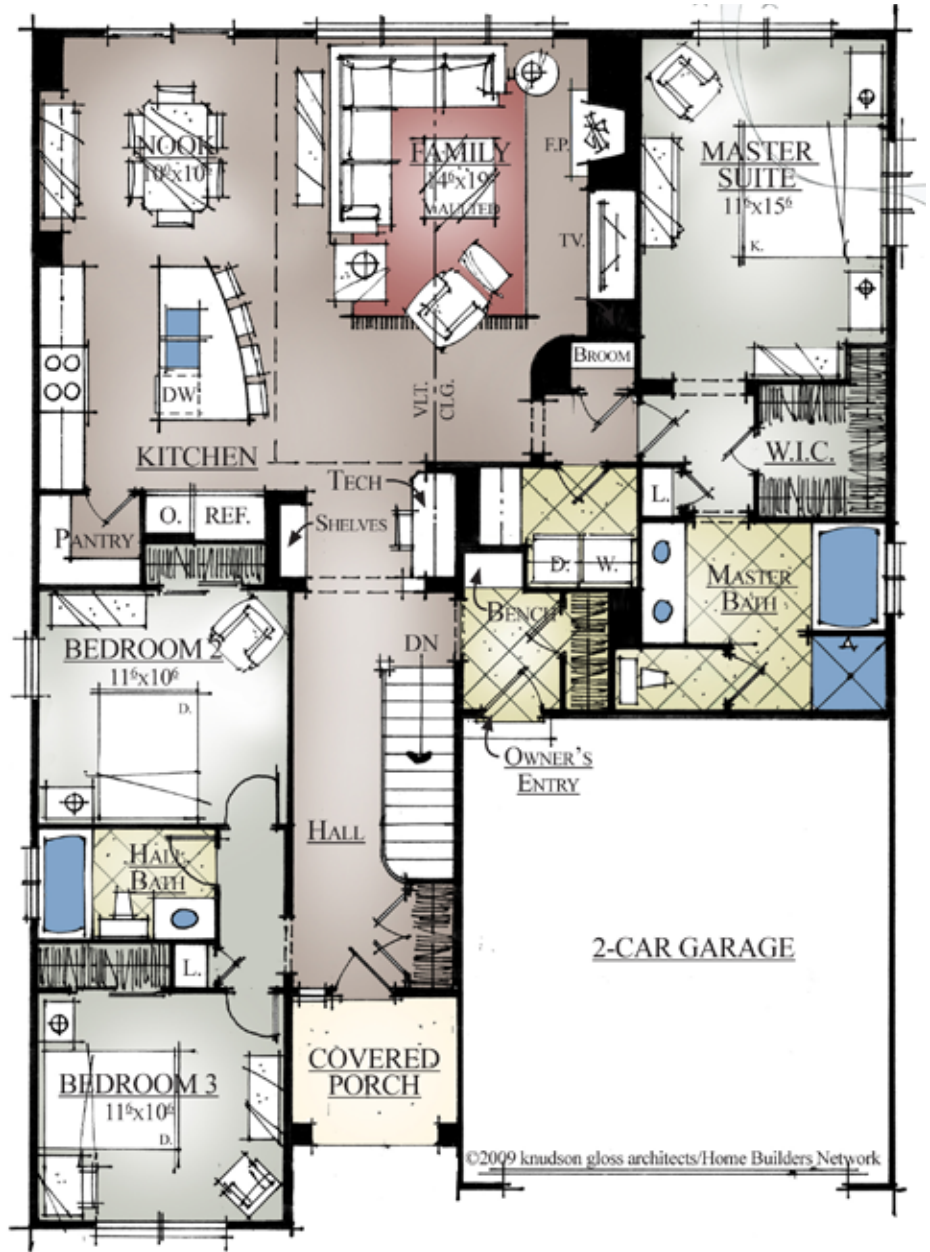
MAIN FLOOR PLAN 0' 4' 8'
