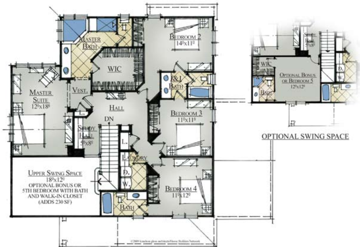
UPPER FLOOR PLAN 0' 4' 8'
